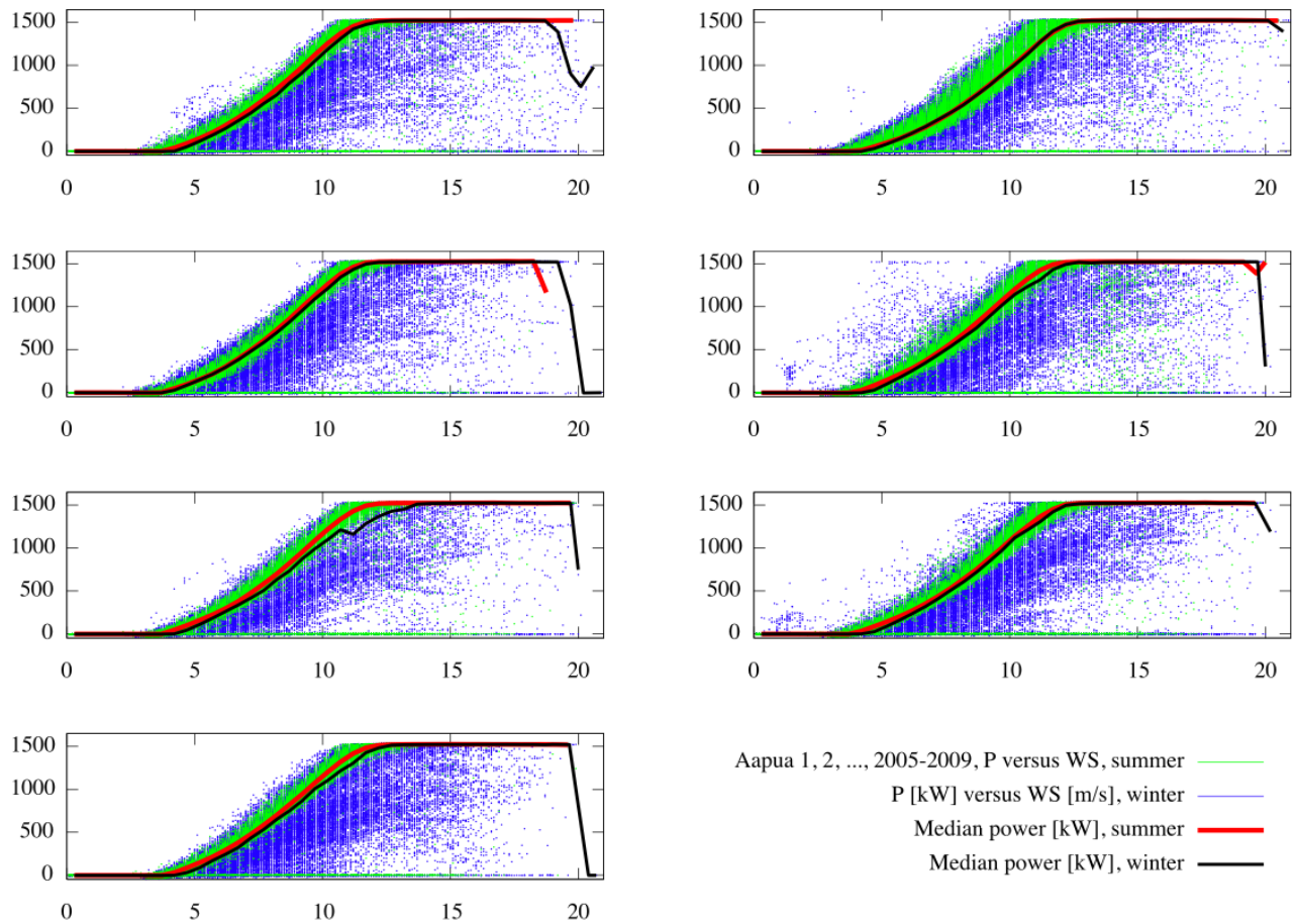
Figure 4: 10-min data plotted for three summers and four winters from October 1st 2005 to March 31st 2009. As data for the winters were plotted first, data for the summers (green dots) are placed on top of the winter data (blue dots). Aapua 1 is top left, Aapua 2 is top right etc.
