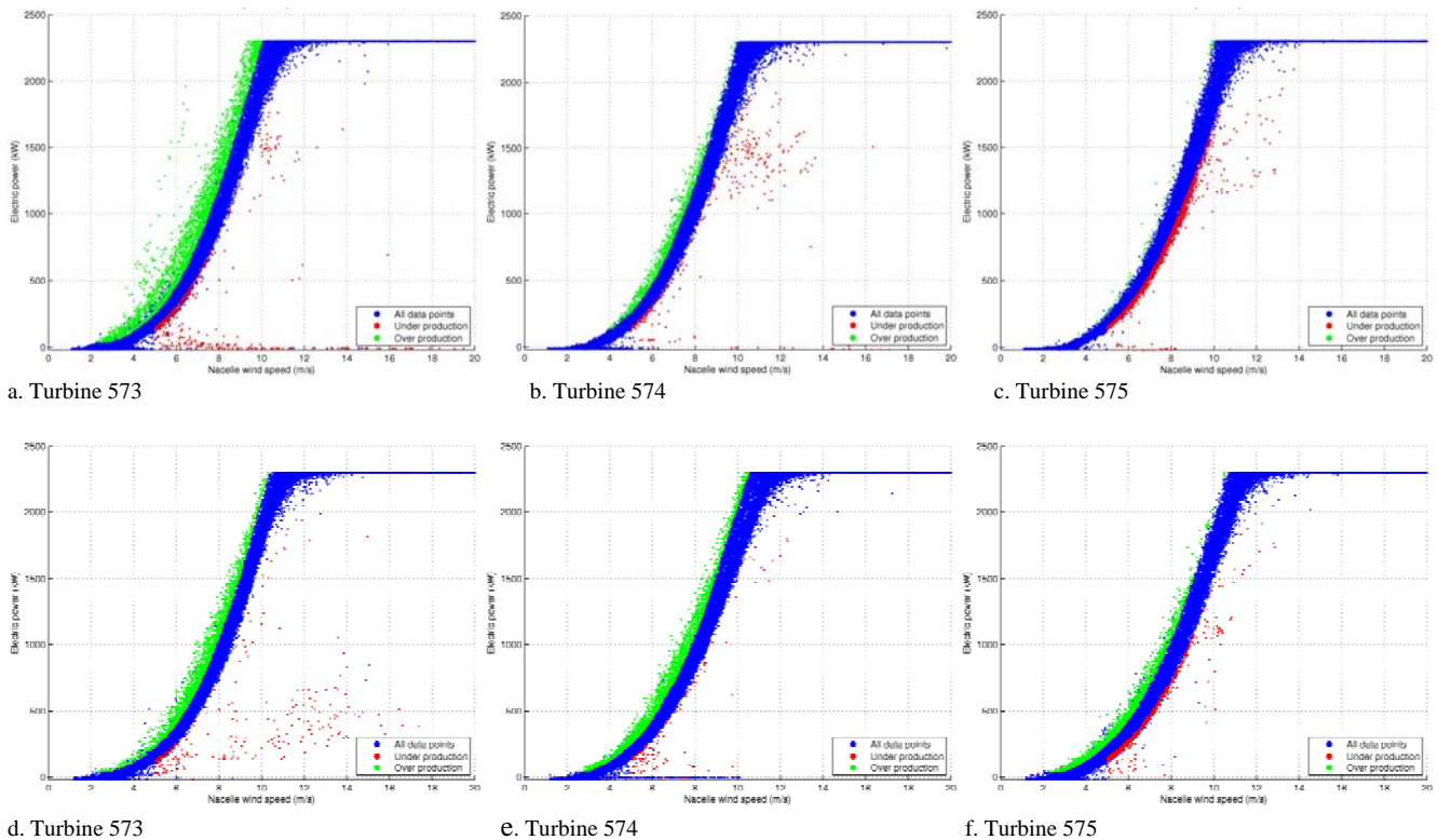
Figure 1: 10 minute production data from Nygårdstjell showing all data in blue, overproduction in green and underproduction in red. Subfigures a, b and c are from 2007-2008, while d, e and f are from 2008-2009.
