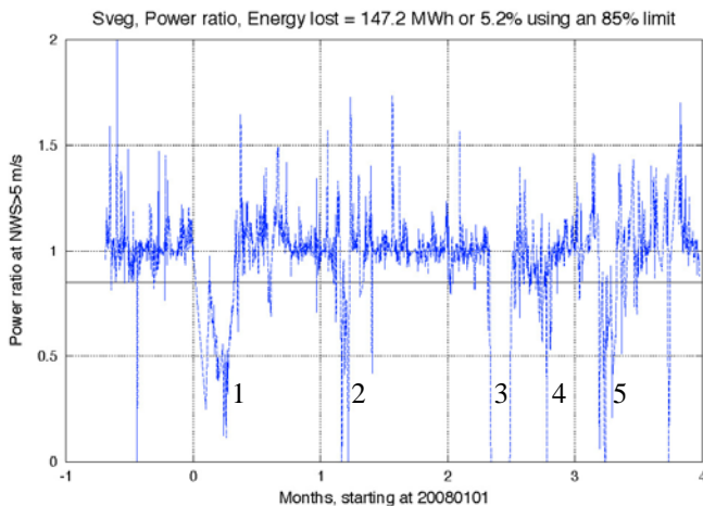
Figure 2: Five periods of icing. The energy production loss due to icing is estimated to be 5% during the period shown. The threshold shown is at 85%.
